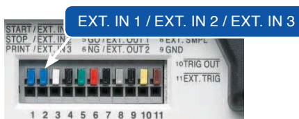
Control terminals
